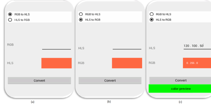
Fig. 1.1 Colour Converter Android application
