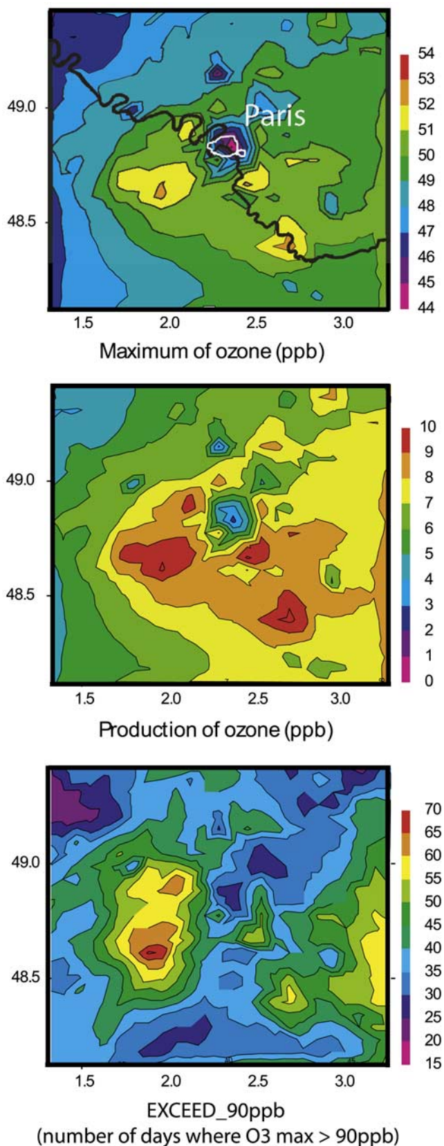
Figure 3. Reference simulations averaged over summers 1998 and 1999 (daily ozone maximum, local ozone production, and EXCEED_90ppb criterion).
