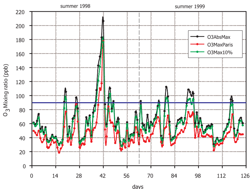
Figure 2. Absolute maximum of ozone (O3AbsMax), maximum of O 3 in Paris (O3MaxParis), and 60 most elevated values of O 3 grid cells (O3Max10%) for individual days of the July–August 1998 and 1999 period.
