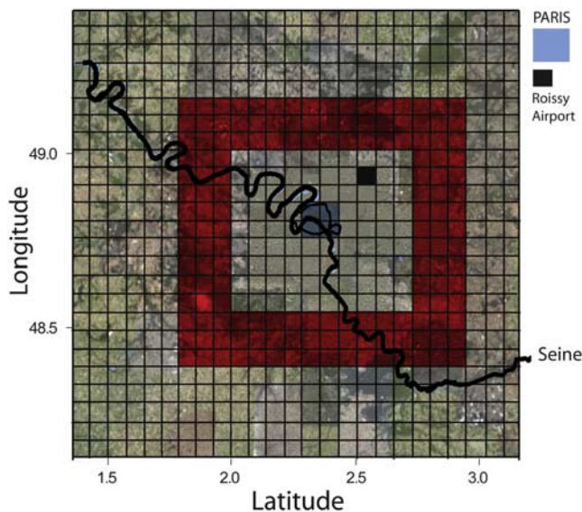
Figure 1. Localization of the grid cells (in red) used for calculation of the O 3 background over the Ile-de-France region.
