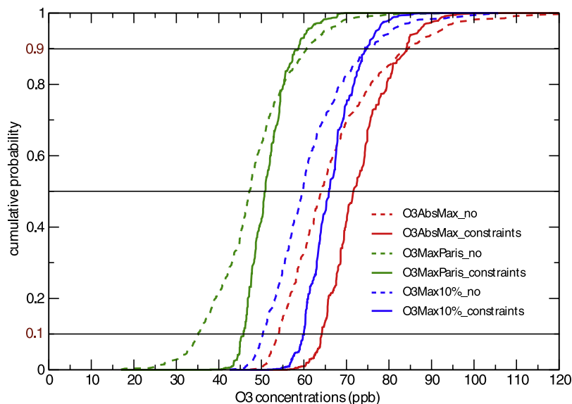
Figure 4. Cumulative probability density function (CPDF) for Monte Carlo simulations without constraints (“no”) and constrained by observations (“constraints”) averaged over summers 1998 and 1999. Red indicates daily absolute maximum of ozone over the model domain (O3AbsMax), green indicates daily maximum of ozone in the Paris area (O3MaxParis), and blue indicates average of the 60 grid cells with the most elevated daily ozone maxima (O3Max10%, intended to reflect the plume average).
