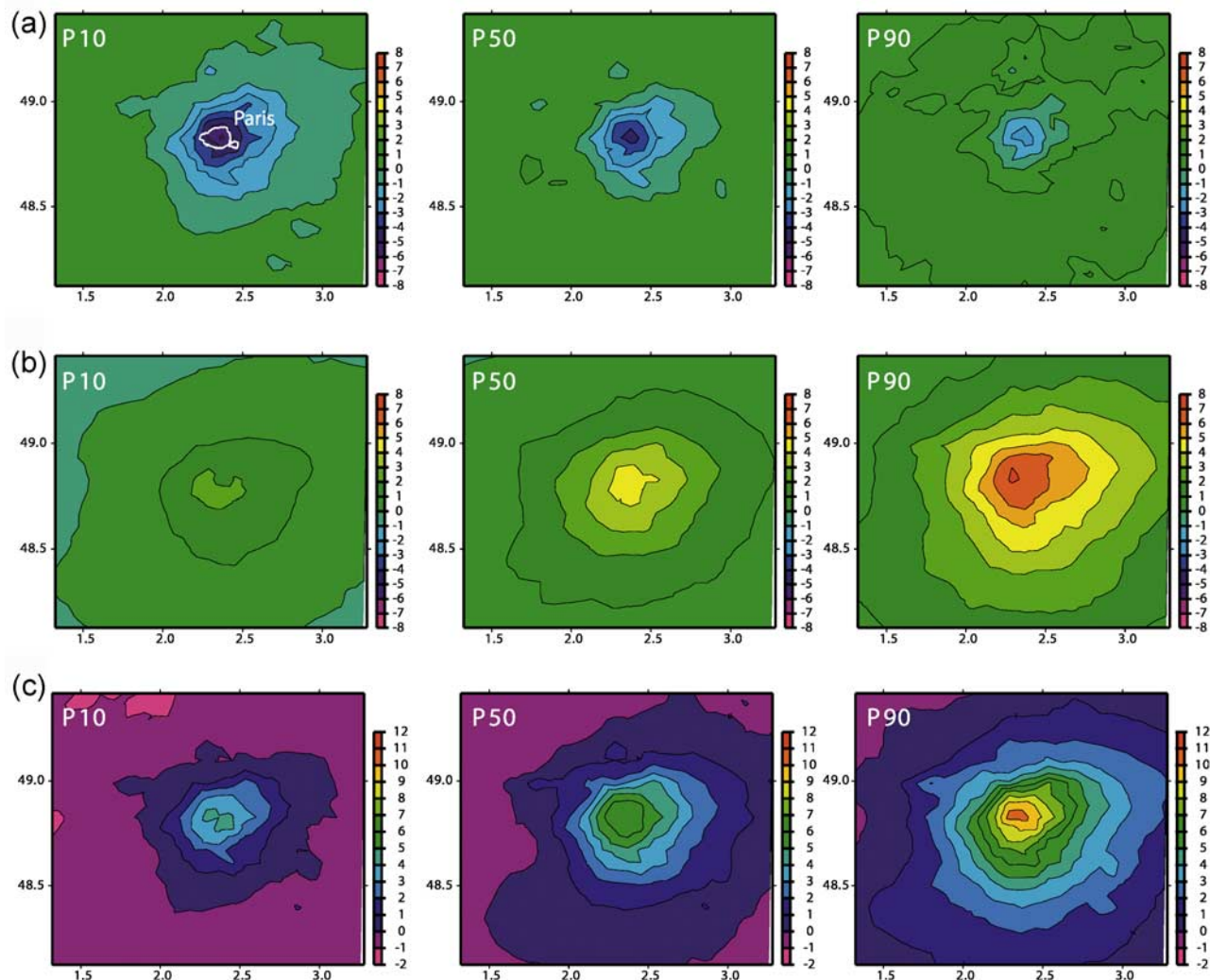
Figure 8. Simulated 10th, 50th and 90th percentiles of the ozone production averaged over summers 1998 and 1999 from constrained Monte Carlo simulations. (a) Baseline emissions minus reduced NO x emissions (−30%), (b) baseline emissions minus reduced VOC emissions (−30%), and (c) reduced NO x emissions (−30%) minus reduced VOC emissions (−30%).
