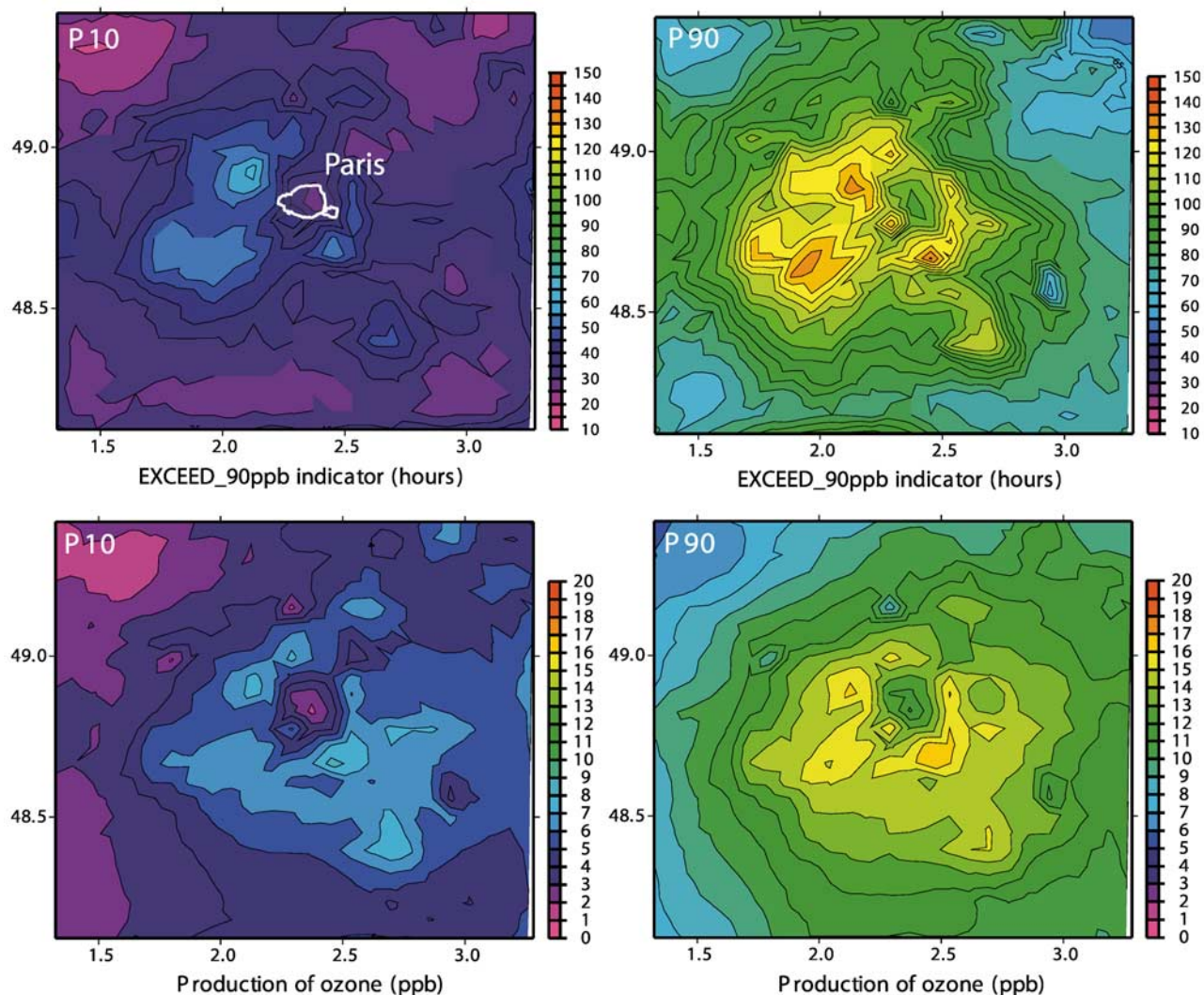
Figure 6. Simulated 10th and 90th percentiles of the production of ozone and of the EXCEED_90ppb indicator averaged or cumulated over summers 1998 and 1999 constrained by observations from the AIRPARIF network.
