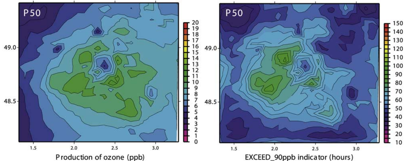
Figure 5. Simulated 50th percentile of the local ozone production and the EXCEED_90ppb indicator averaged or cumulated over summers 1998 and 1999 from (top) constrained or (bottom) unconstrained Monte Carlo simulations.
