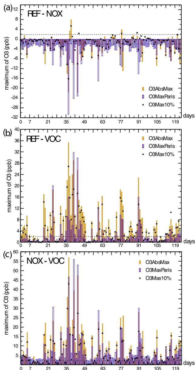
Figure 7. Difference of the daily absolute maximum of ozone ( O_3\text{AbsMax} ), of the ozone in the Paris area ( O_3\text{MaxParis} ) and of the 10th of the most elevated ozone values ( O_3\text{Max10\%} ) between (a) baseline emissions minus reduced \text{NO}_x emissions ( -30\% ), (b) baseline emissions minus reduced VOC emissions ( -30\% ), and (c) reduced \text{NO}_x emissions ( -30\% ) minus reduced VOC emissions ( -30\% ).
