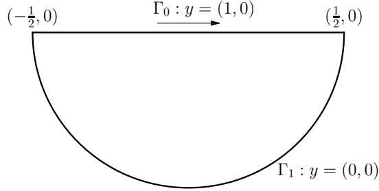
Fig. 2 Semi-disk geometry.
