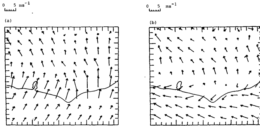
FIG. 12. Simulated wind field at 1500 LST on 6 January 1979 at (a) 5 m, and (b) 2000 m. (Velocity scale included in the figure.)
