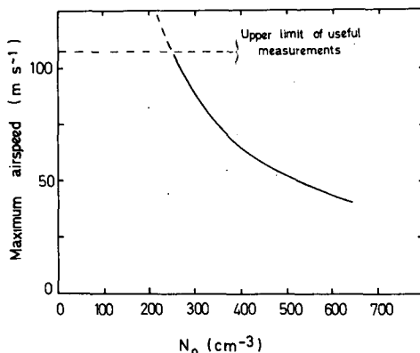
FIG. 10. Estimation of the values of the maximum airspeed beyond which the ASSP measurements cannot be used as a function of the true droplet concentration ( N_0 ).
