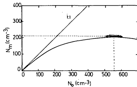
FIG. 7. Plot of the ASSP measured droplet concentration ( N m ) as a function of the true droplet concentration ( N 0 ), N_m = N_0 \exp(-\alpha N_0) , \alpha = 0.00018 \text{ cm}^3 (see text).
