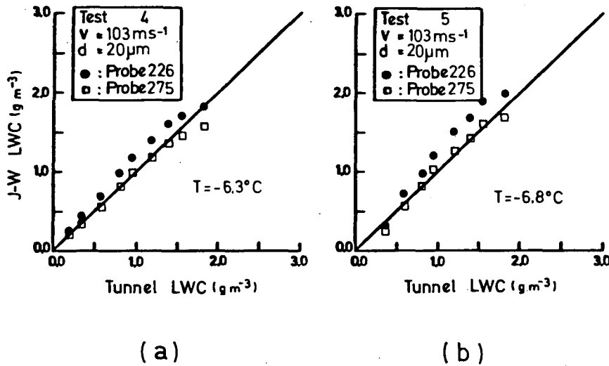
FIG. 3. Despite identical wind tunnel conditions, the responses of the two probes are different between (a) test 4 and (b) test 5. Note also the saturation of the probe responses for LWC > 1.5 g m -3 .
