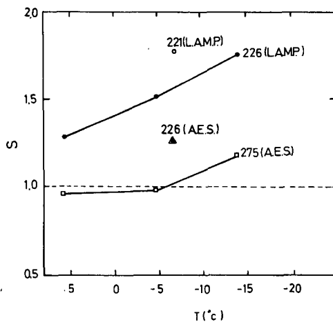
FIG. 5. Values of the slopes of regression lines ( S ) as a function of static temperature ( T ) for different sensor heads. Results of the tests performed at 51 m s -1 are shown. The symbols in parentheses indicate the control unit with which the sensor head has been recorded.
