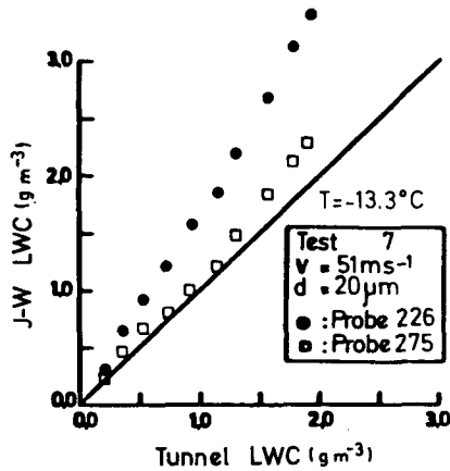
FIG. 4. Test 7. Overestimation of the probes for an airspeed of 51 m s -1 and a temperature of -13.3°C.
