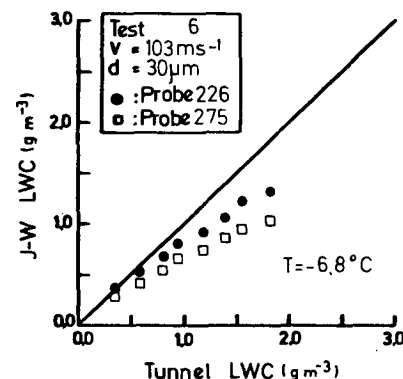
FIG. 2. Test 6. The figure shows the underestimation of the two probes for median volume diameter of 30 \mu m.
