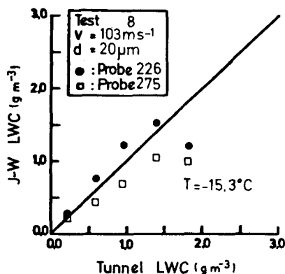
FIG. 1. Johnson-Williams liquid water content vs wind tunnel liquid water content. Values plotted are ~30 s averages. The test number, the airspeed, the wind tunnel median volume diameter, the static temperature and sensor head numbers are also indicated with the 1:1 line. Test 8. This figure shows the Johnson-Williams underestimation due to the icing of the probe for LWC > 1.5 g m -3 .
