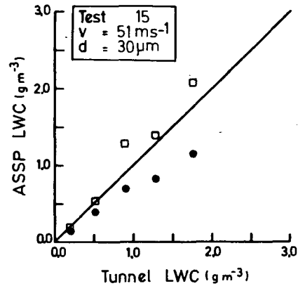
FIG. 6. Test 15. ASSP liquid water content vs wind tunnel liquid water content. Values plotted are \sim 30 s averages; \bullet symbols correspond to uncorrected values; \square symbols correspond to corrected values.
