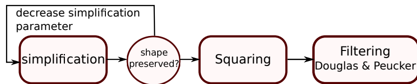
Figure 11: Process used for automatic building generalization.
