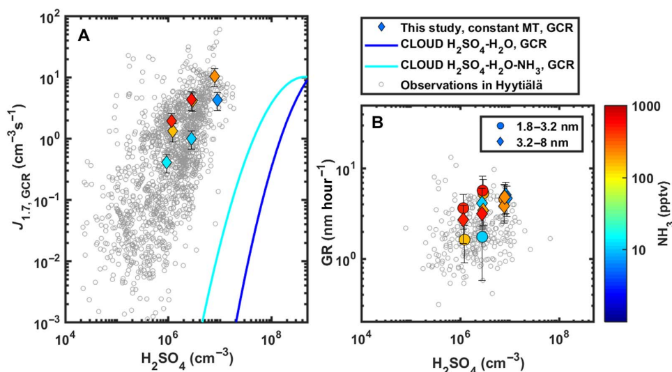
Fig. 3. Nucleation and GRs at CLOUD compared to atmospheric observations in Hyvitiälä. Here, we chose a series of experiments with constant MT/NO x ratio (ca. 0.6, NO/NO 2 = 7%), while H 2 SO 4 and NH 3 concentrations were varied across the range relevant for boreal forest. (A) Nucleation rates ( J_{1.7} ) at CLOUD (colored points) and ambient observations in Hyvitiälä (5, 8) (gray circles). The blue and cyan lines represent binary (H 2 SO 4 -H 2 O) and ternary (H 2 SO 4 -H 2 O-NH 3 , 7 < [NH 3 ] < 40 pptv) nucleation, respectively, based on earlier CLOUD data (27), while the pure biogenic nucleation rate at similar MT/NO x ratio would be <1 cm -3 s -1 (fig. S3). (B) GRs of 1.8- to 3.2-nm-sized and 3.2- to 8-nm-sized particles in the same experiments compared to observations of initial GR in Hyvitiälä (40).
