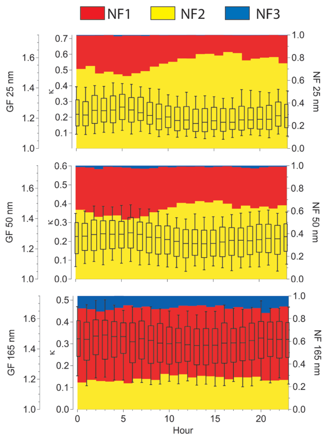
Figure 6. Diurnal variation of hygroscopic growth factor (GF), kappa value ( \kappa ) and number fractions (NF) measured at RH90 for particles in the nucleation mode (top panel), Aitken mode (middle panel) and accumulation mode (bottom panel). The figure shows the median GF value, with the bottom and top sides of the box giving the 25th and 75th percentiles, and the extremities the 10th and 90th percentiles. The coloured bars illustrate the NF of particles found in each hygroscopic mode.
