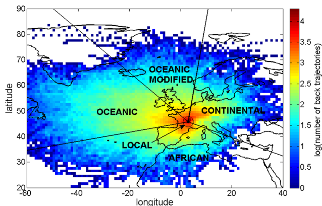
Figure 8. Back trajectories of air masses measured at the Puy de Dôme over the measurement period September 2008–December 2012, calculated from the HYSPLIT model.
