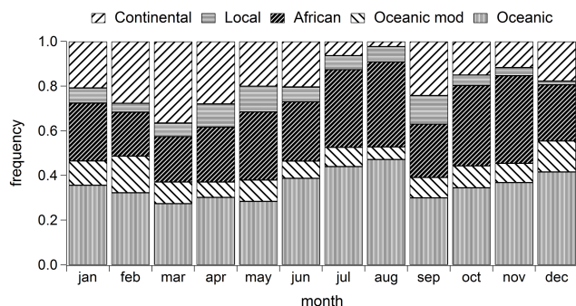
Figure 9. Seasonal variations in back trajectories of air masses measured at the Puy de Dôme over the measurement period September 2008–December 2012.
