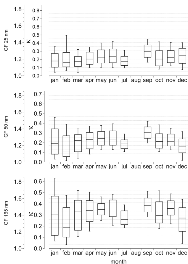
Figure 3. Monthly variation of hygroscopic growth factors (GFs) and kappa values ( \kappa ) measured at RH90 for particles in the nucleation mode (top panel), Aitken mode (middle panel) and accumulation mode (bottom panel). The figure shows the median GF and \kappa value, with the bottom and top sides of the box giving the 25th and 75th percentiles, and the extremities the 10th and 90th percentiles.
