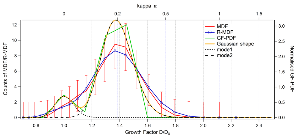
Figure 1. Example of a bimodal growth factor distribution function measured at RH90. The red line refers to measured particle counts, i.e. the MDF (left axis), and the green line is the GF-PDF (right axis). The black dotted lines and the yellow line are the results of super-positioning multiple Gaussians over the GF-PDF obtained from the TDMAinv program (right axis). The bottom axis gives the growth factor GF and the top axis shows the corresponding kappa value \kappa . Error bars indicate the estimated counting uncertainty of the measurements.
