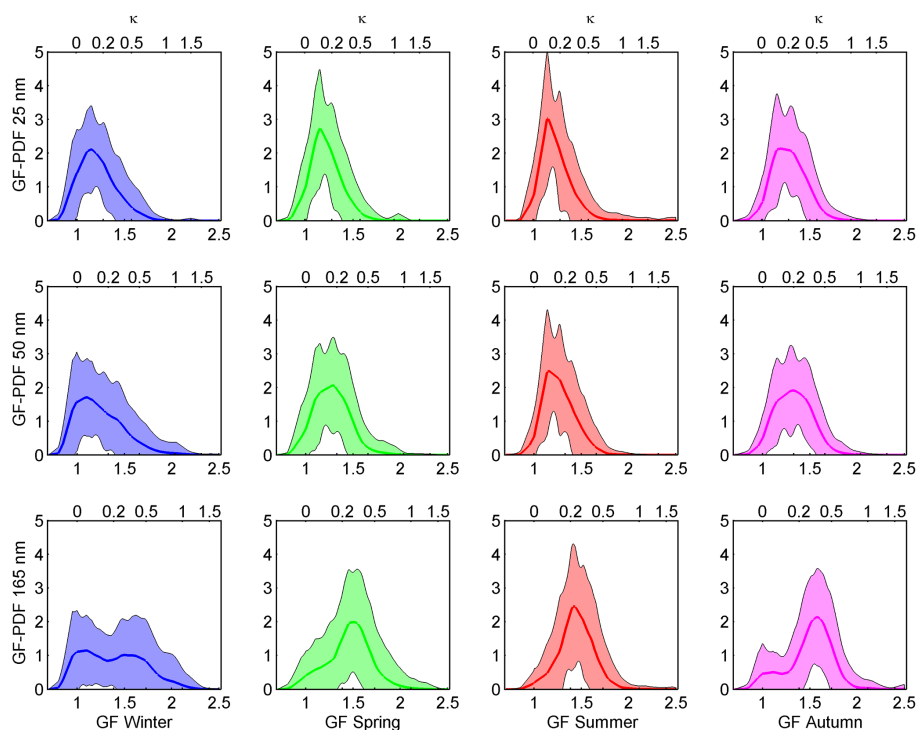
Figure 4a. Average GF-PDFs and their standard deviations for particles in the nucleation mode (top panels), Aitken mode (middle panels) and accumulation mode (bottom panels), split by season and measured at RH90. The bottom axis gives the growth factor GF and the top axis shows the corresponding kappa value \kappa .
