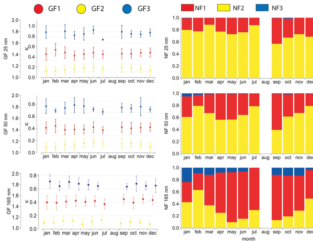
Figure 5. Annual variation of hygroscopic growth factor (GF), kappa value ( \kappa ) (left panels) and number fractions (NF) (right panels) measured at RH90 for particles in the nucleation mode (top panels), Aitken mode (middle panels) and accumulation mode (bottom panels). The coloured bars show the average NF of each hygroscopic mode and the markers give the average GF in each mode, including standard deviations.
