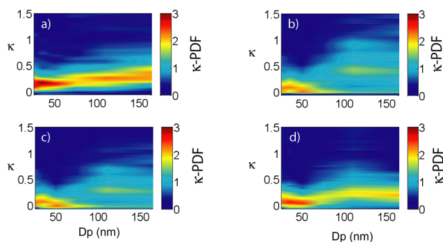
Figure 4b. Average \kappa -PDFs as a function of particle diameter, split by season and measured at RH90: (a) represents winter, (b) spring, (c) summer and (d) autumn.
