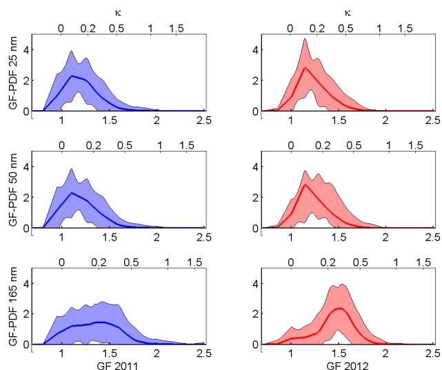
Figure 2a. Yearly average GF-PDFs and their standard deviations for particles in the nucleation mode (top panels), the Aitken mode (middle panels) and the accumulation mode (bottom panels), measured at RH90. The bottom axis gives the growth factor GF and the top axis shows the corresponding kappa value \kappa .
