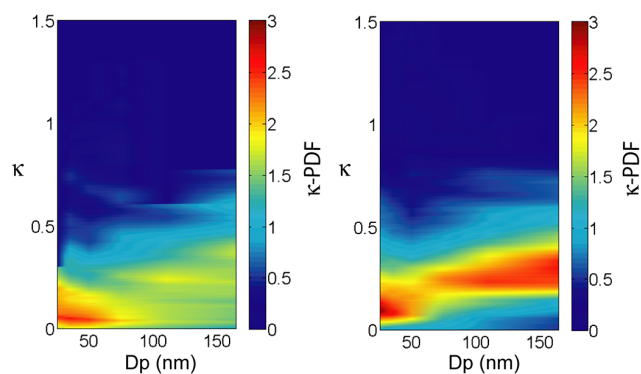
Figure 2b. Yearly average \kappa -PDFs as a function of particle diameter, measured at RH90, for measurement years 2011 (left panel) and 2012 (right panel).
