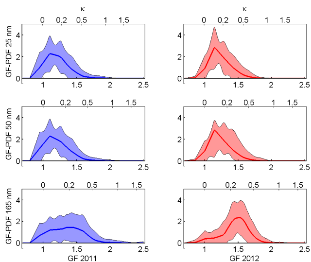
Figure 2a. Yearly average GF-PDFs and their standard deviations for particles in the nucleation mode (top panels), the Aitken mode (middle panels) and the accumulation mode (bottom panels), measured at RH90. The bottom axis gives the growth factor GF and the top axis shows the corresponding kappa value \kappa .
