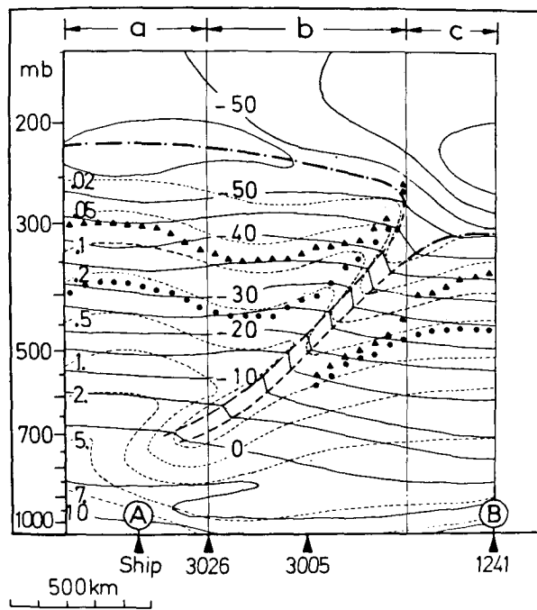
FIG. 12. Vertical cross-section AB. See legend of Fig. 2. Black circles and triangles are for the altitudes of the CFP and WFP peaks, respectively, as determined by LOWTRAN IV model (as Fig. 10). For zones a , b and c see text.
