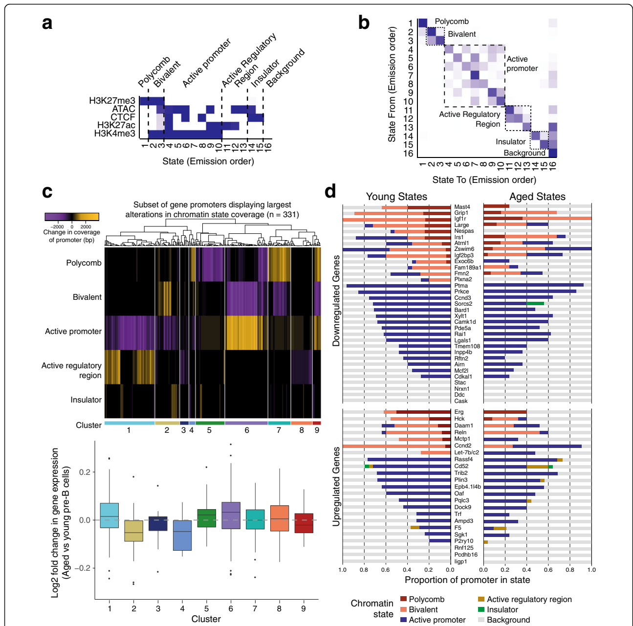
Fig. 6 Integrated chromatin state analysis in pre-B cells identifies age-related changes. a Emission parameters learnt by the Hidden Markov Model in chromHMM analysis. It shows the likelihood of emitting each of the 5 marks used in this analysis at any given chromatin state. b Transition parameters learnt by the HMM in chromHMM analysis: given the current chromatin state (at a specific 200-bp genomic region), how likely is it that the adjacent 200-bp region will be in any of the 16 inferred states. Dashed blocks show states that transit to each other more frequently suggesting a more biologically meaningful chromatin state, thus driving our clustering into 6 states: Polycomb, Bivalent, Active Promoter, Active Regulatory Region, Insulator, and Background. c Top : Heatmap showing the change in the occupancy (bp) of each regulatory chromatin state over gene promoter regions (2500-bp up- and downstream of TSS), for a subset of genes showing the largest magnitude changes. Genes are hierarchically clustered based on their correlation and assigned to 9 clusters showing distinct patterns. Bottom : Log2 fold change in expression of genes in each cluster, in aged versus young pre-B cells. Dashed line indicates unchanged gene expression. To better display the data, some outliers are not displayed. d Fraction of promoter regions (defined as for c ) of DEGs occupied by each of the 6 chromatin states in young and aged pre-B cells. Note that Let-7b/c2 refers to the potential regulatory region/alternative promoter over which we have observed significant alterations in chromatin marks
