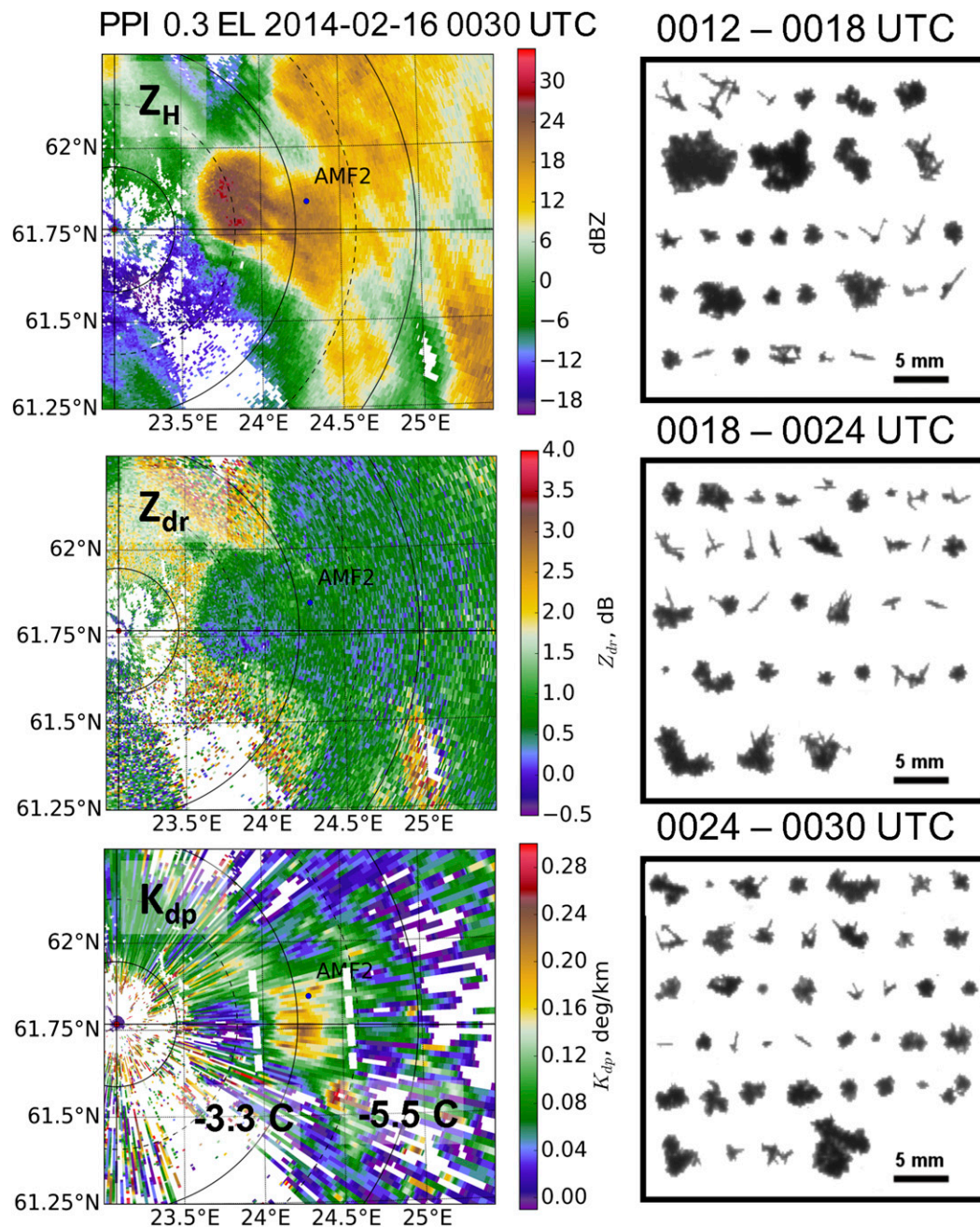
FIG. 7-7. (left top to bottom) Finnish Meteorological Institute Ikaalinen radar plan position indicator observations of equivalent reflectivity Z_H , differential reflectivity Z_{dr} , and specific differential phase of a snow storm that took place on 15–16 Feb 2014. The enhanced specific differential phase signature K_{DP} , appears in the temperature region between -3^\circ and -5^\circ\text{C} . The signature is observed close to the ground and surface precipitation observations indicate presence of columnar crystals, densely rimed particles and aggregates of columnar crystals, as shown in the right column.
