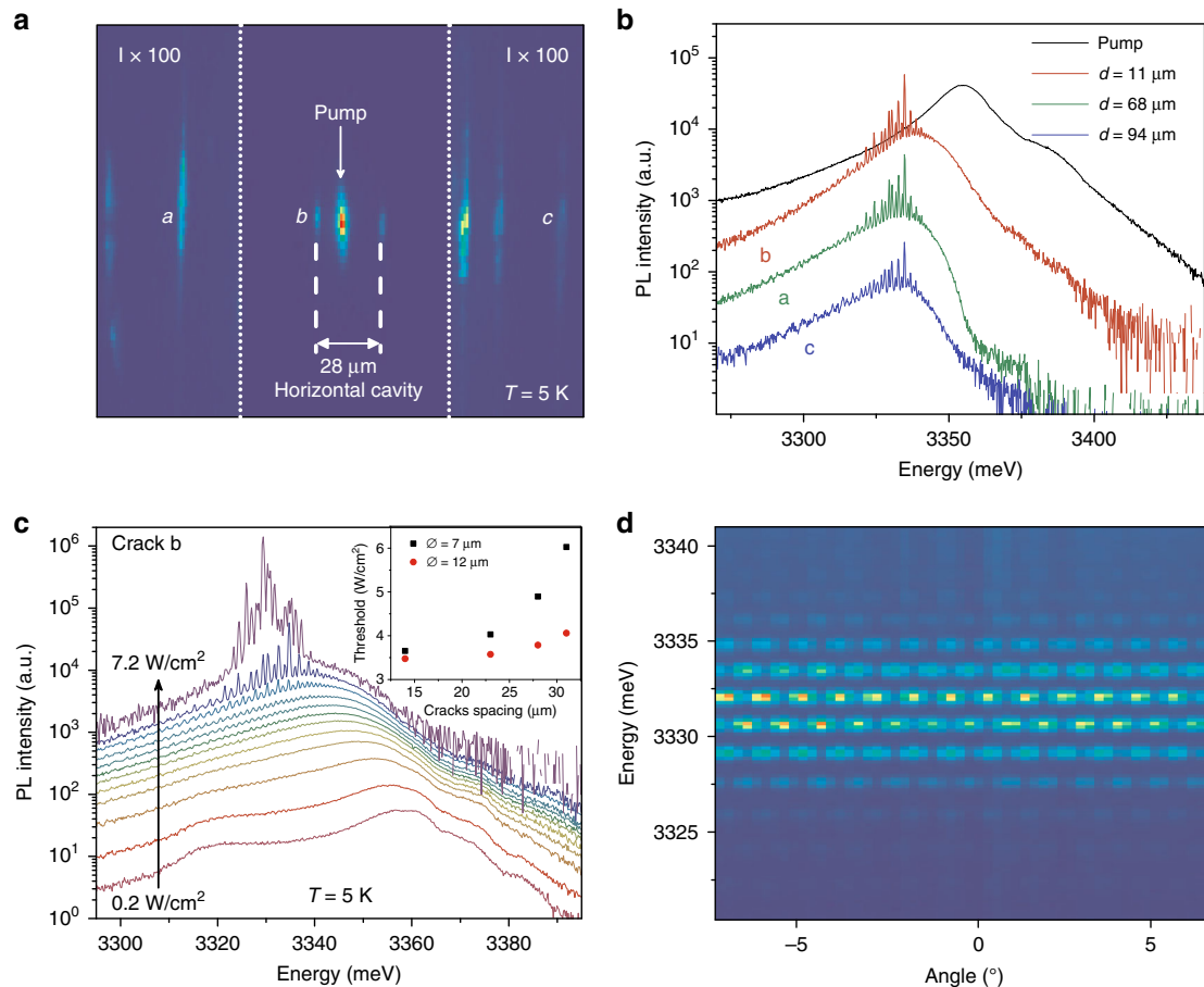
Fig. 3 Sample W2. a Real space emission at 5K. The intensity ( I ) of the two lateral regions is magnified by 100. b Emission spectra from the pump region and from the cracks labeled “a”, “b”, and “c” in Fig. 3a. d is the distance between the crack and the center of the excitation spot. c Emission of the crack “b” vs. pumping power, showing the emergence of the Fabry-Perot modes of the horizontal cavity together with the onset of lasing (power dependence is shown in Supplemental Material). The inset shows the threshold values vs. the cavity size for two different pump diameters. d Far-field image zoomed in onto the fringes resulting from the interference of the emission from two distant cracks, demonstrating their mutual coherence
