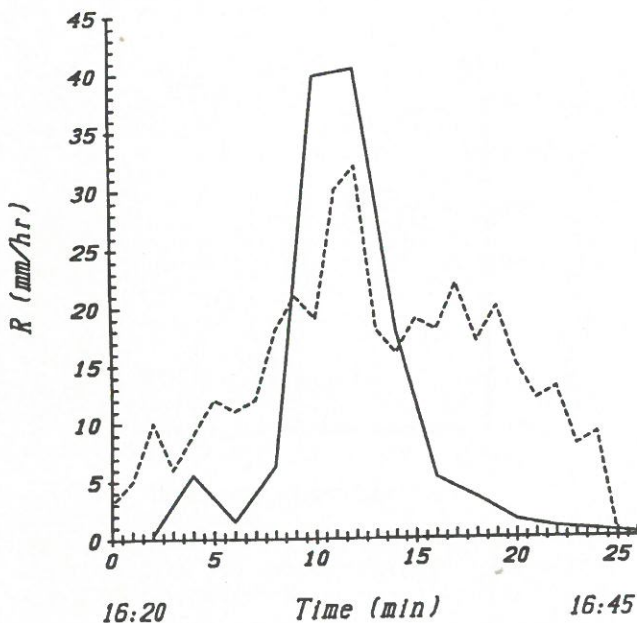
Figure 6 Comparison of the observed (dashed line) and computed (solid line) rain rate on the ground at the point Y = 10 \text{ km} ( P(0./10.) ) in the model domain of cloud-2.
