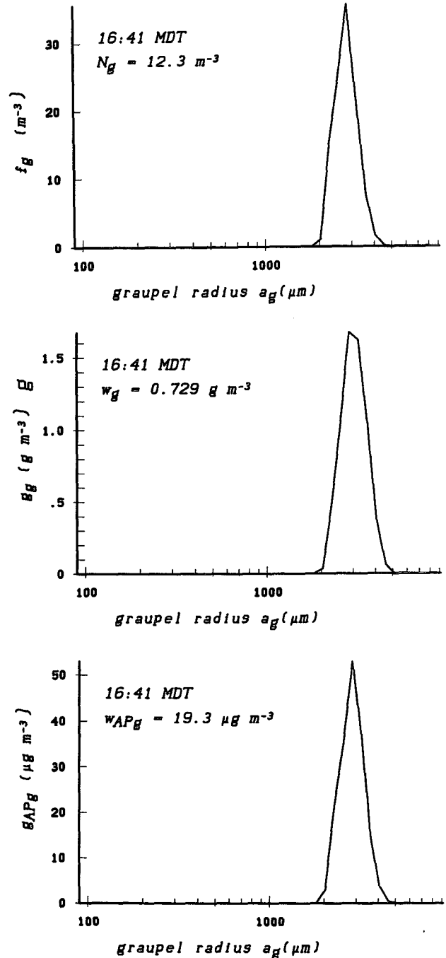
FIG. 5. For X = 18 km, Z = 4925 m ASL, and for 1641 MDT ( t_w = 41 min). (a) Number density distribution function of graupel f_g(a_g) , N_g = total number of graupel. (b) Graupel mass density distribution function g_g(a_g) , w_g = total mass of graupel. (c) Aerosol mass density distribution function within graupel g_{APg}(a_g) , w_{APg} = total AP mass within graupel. The density distribution functions are displayed per logarithmic radius interval.
