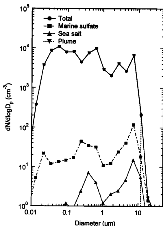
Figure 9. Predicted in-cloud particle and droplet size distribution for track air in the clean marine case (JDT 180). Symbol definitions are the same as in Figure 8.
