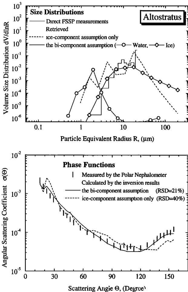
Figure 4. The same as in Fig.1 but for mixed-phase cloud obtained during NEPHELOMETER '97 airborne measurements.
