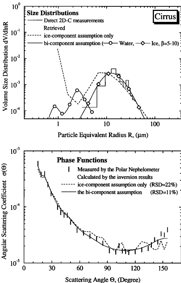
Figure 2. The same as in Fig.1 but for ice cloud obtained during CIRRUS'98 airborne measurements.
