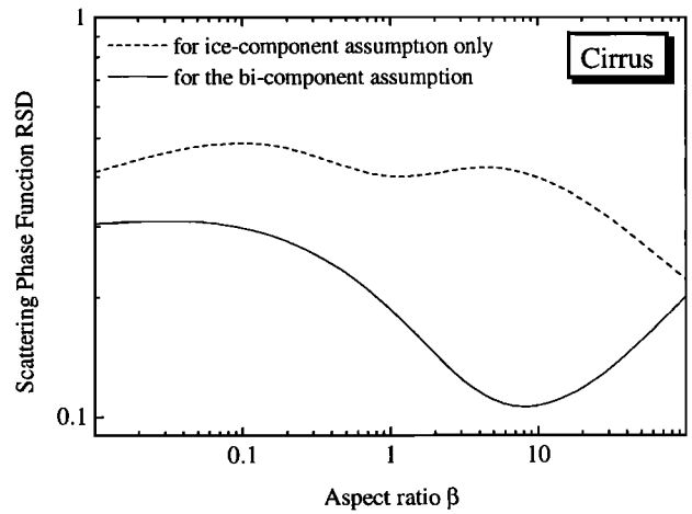
Figure 3. Scattering phase function RSD versus the aspect ratio of ice crystals fed in solving the inverse problem with respect to retrieval of equivalent crystal size distribution for cirrus (ice crystal assumption only).
