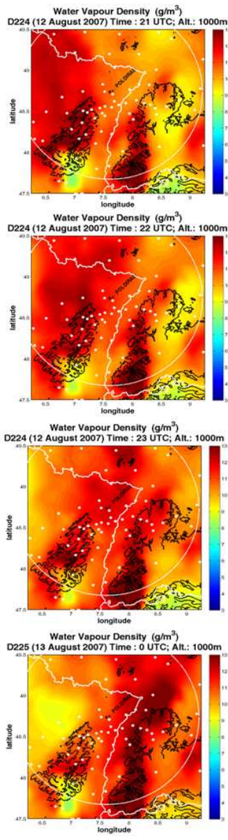
POLDIRAD reflectivity PPI observations on August 12, 2007 at 21:00, 22:00, 23:00, and August 13, 2007 at 00:00 UTC (IOP 15) respectively (left column) and GPS tomography horizontal water vapour density fields at the 1000 m height layer for the same times (right column). The radar reflectivity scale goes from -10 to 60 DBz. The water vapour density scale goes from 3 to 13 \text{g/m}^3 .
