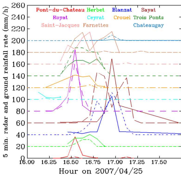
Fig. 4. Time series of 5 min radar and ground rainfall rates for the different rain-gauge sites. Each successive site is augmented by 20 mm/h for visibility. Dash lines for rain gages observations, solid lines for X-band radar estimations.
