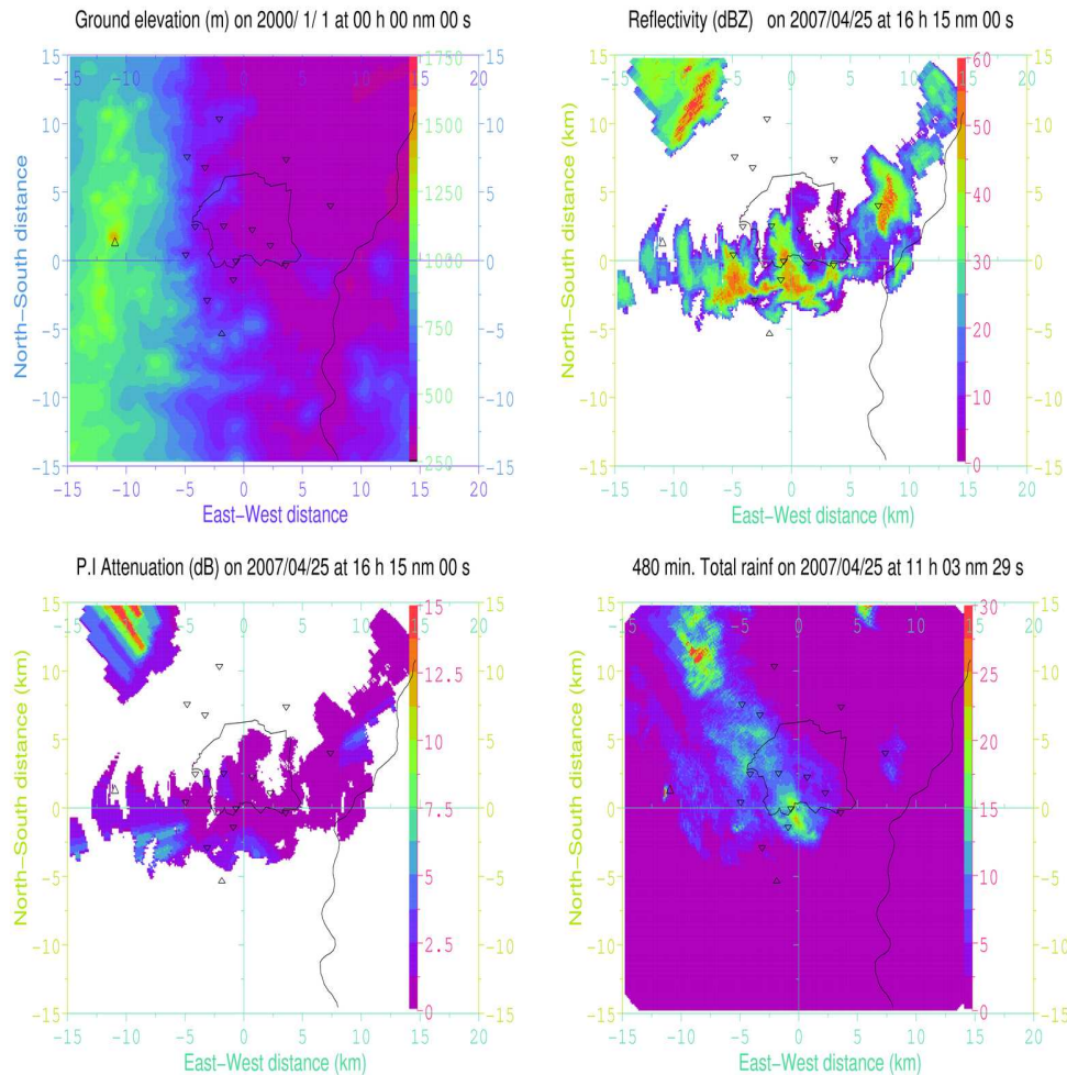
Fig. 3. (a) Radar environment orography with the Puy de Dôme to the West and the markers to identify the rain-gages location while the solid lines indicate the contour of Clermont-Ferrand and the Allier river; (b) Reflectivity display of the X-band scanning radar; (c) Estimated Path Integrated Attenuation display for the X-band scanning radar; (d) Derived 8 h accumulated precipitation display with the X-band scanning radar.
