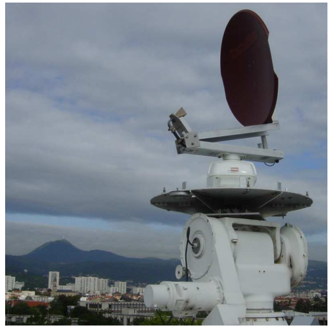
Fig. 1. View of the Clermont-Ferrand X-band precipitation radar without its protective radome. Parts of the city of Clermont-Ferrand and the Puy de Dôme are visible in the background.
