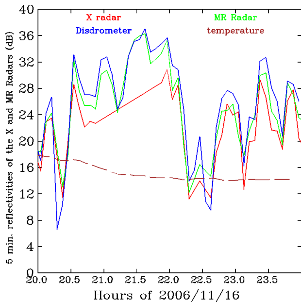
Fig. 2. Reflectivity from the X-band radar (red curve), the MRR (green curve) and estimated from the disdrometer measurements (blue curve) while the surface temperature is provided by a dash line.
