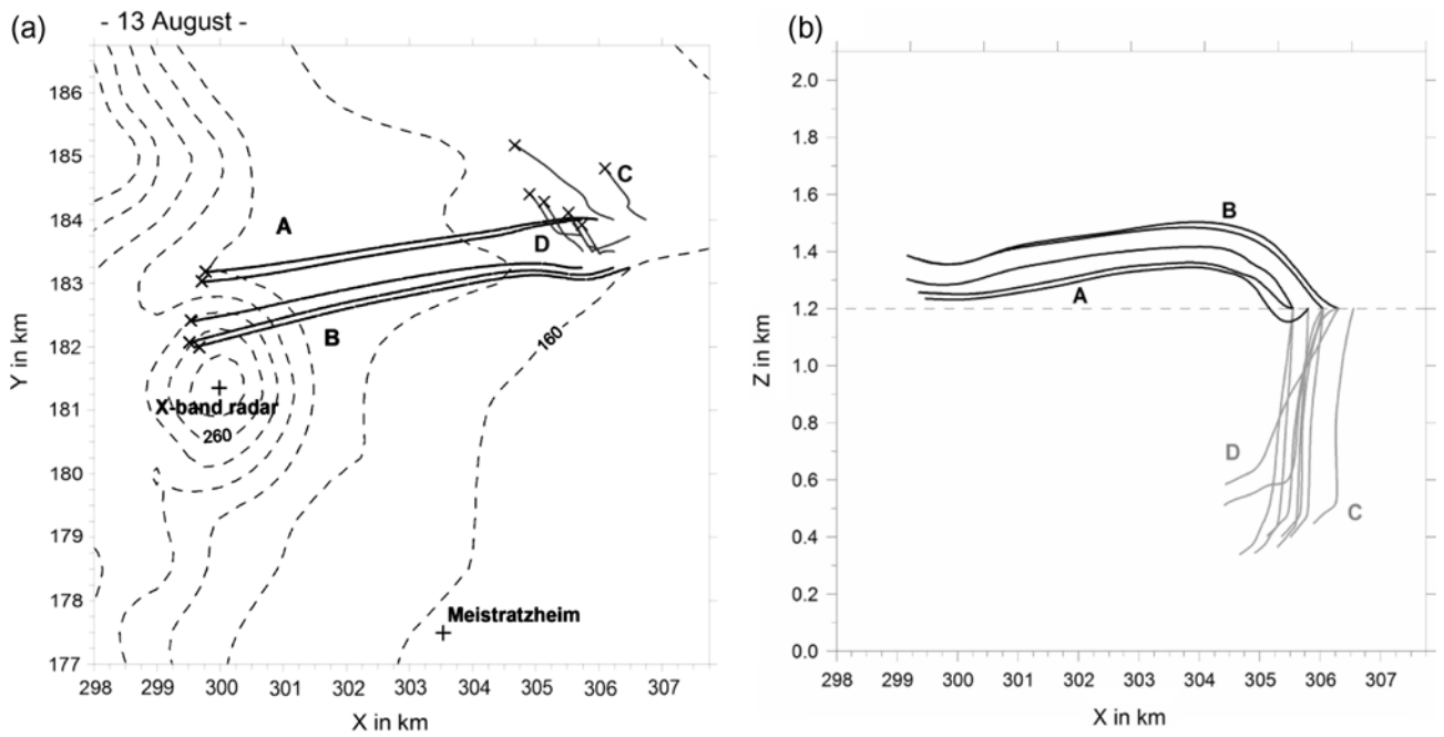
Figure 7: Horizontal (a) and vertical (b) cross section of the 20 min back-trajectories that track the air parcels that trigger the convective system observed on August 13. The area of this study is represented by the dashed black line on the Fig. 4e. The letters are used to easier understand the position of the different back-trajectories and the crosses represent the origin points of the back-trajectories.
