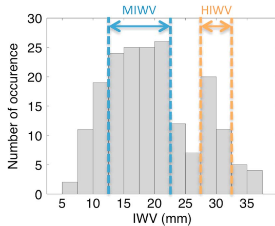
Figure 3. Distribution of the IWV measured 20 min before the peak of precipitation for the 191 cases considered in this study. The medium IWV (MIWV) mode corresponds to IWV between 12.5 and 22.5 mm (100 cases), whereas the high IWV (HIWV) mode corresponds to IWV between 27.5 and 32.5 mm (31 cases).
