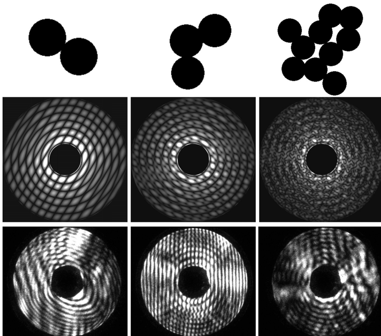
FIG. 15. Simulation of diffraction patterns from frozen droplet aggregates using 2D Fourier transform on idealized ice spheres. (top) Simulations were made for aggregates of 2, 3, and 10 spheres, where the sizes of the individual spheres were kept constant. (middle) The simulation results. (bottom) Diffraction patterns of real aggregated frozen droplets found in a convective outflow over Texas during the MACPEX campaign.
