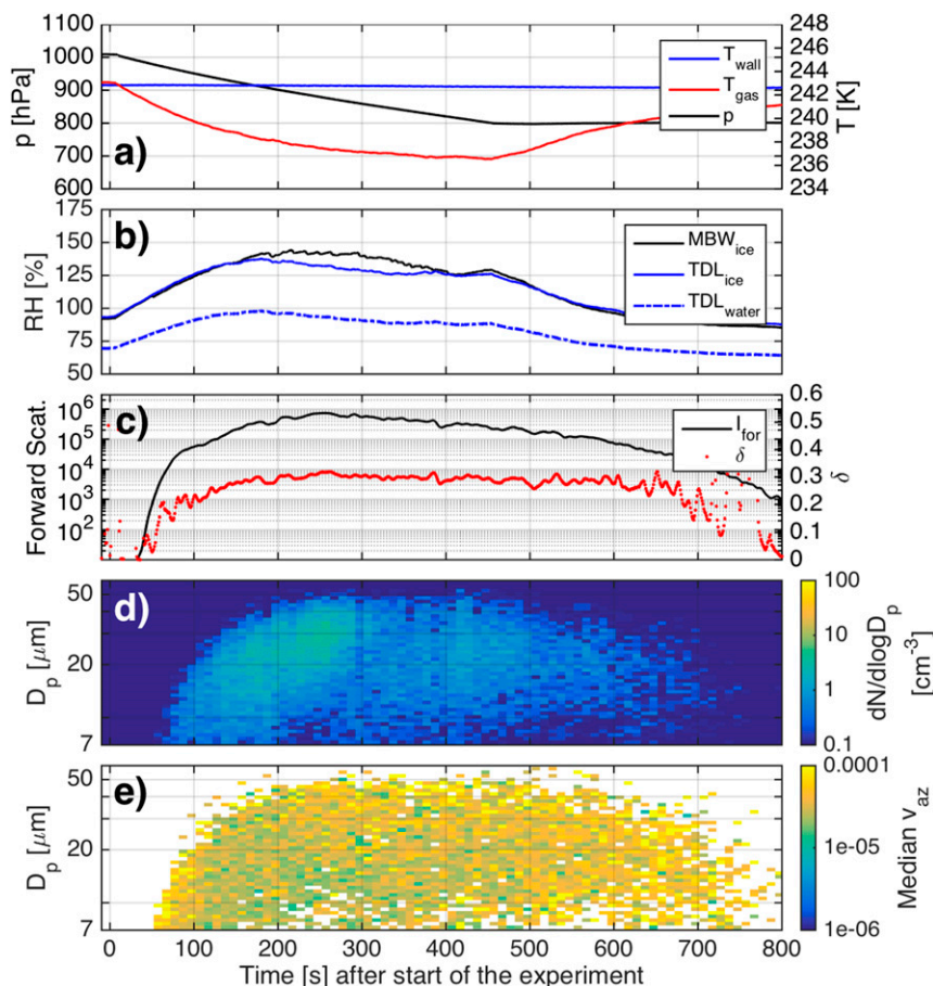
FIG. 8. Simulation of a convective system, where the ice particles nucleate through vapor phase (experiment 24). The experiment was started with 16\text{ cm}^3 of Argentinean soil dust particles and a pumping speed of 60% that led to an initial cooling rate of -1.5\text{ K min}^{-1} . (a) The pressure of the chamber (black line) as well as the chamber and wall temperatures (red and blue lines, respectively). (b) The total water measured with MBW (black line) and the interstitial water with respect to ice (blue solid line) and water (blue dashed line) measured with TDL. (c) The forward-scattering intensity (black line) and the depolarization ratio were measured for cloud particles in the middle of the chamber. (d) The PPD-2K size distribution. (e) The size-segregated median variance of the 2D scattering patterns.
