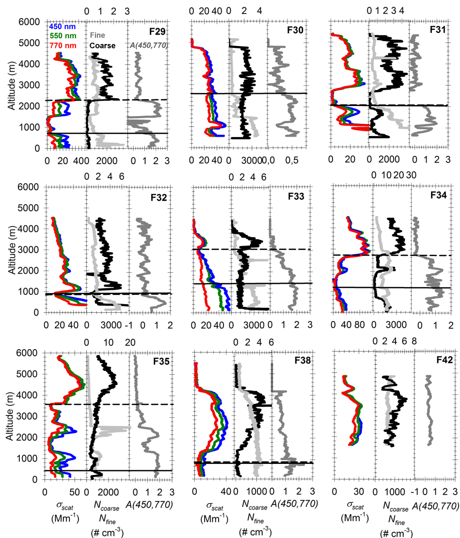
Figure 5. Vertical profiles of the aerosol scattering coefficient \sigma_{\text{scat}} at \lambda = 450, 550 and 770\text{ nm} (blue, green and red), the particle number concentration in the submicron N_{\text{fine}} (light grey) and the supermicron N_{\text{coarse}} (dark) size ranges and the scattering Ångström exponent \text{\AA} calculated between 450 and 770 nm (dark grey). N_{\text{coarse}} is plotted using the upper horizontal axis. The top of the boundary-layer Z_b and the wind shear level Z_s are indicated by a horizontal and dashed line respectively. The height of Z_b was situated below the minimum flight level in F30 and F42. The height of Z_s was situated below the minimum flight level in F42. Data were corrected for standard temperature and pressure using T = 20^\circ\text{C} and P = 1013.25\text{ hPa} .
