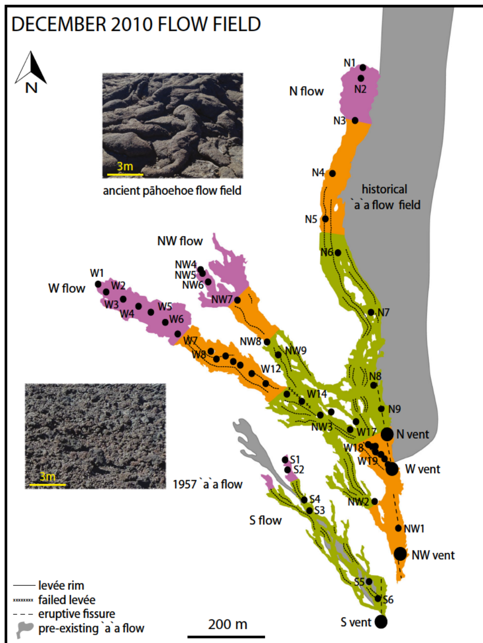
Fig. 3 Structural map of the December 2010 flow field, including eruptive fissures, vents, levée rims, and substrate photos, as well as flow system architecture; sample locations are also plotted. Single channel flow sections are visualized in orange, braided flow sections are displayed in green, and dispersed flow sections are shown in purple
