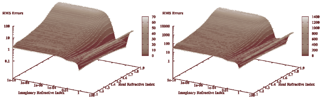
Figure 2. RMS errors functions plotted in the case of absorbing particles m = 1.3 + i . Left panel is the test without measurement errors, right panel is the test with measurement errors \varepsilon = 0.1 .
