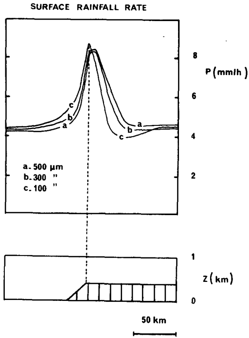
FIG. 4. Surface rainfall rate for different values of the mean seeding raindrop diameter, D_{sr} .
