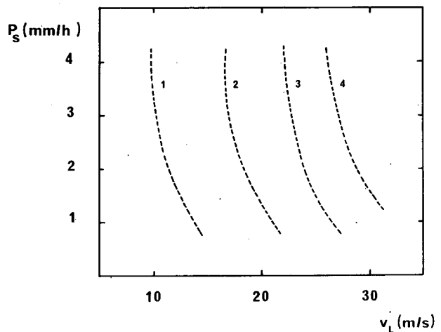
FIG. 10. Orographic enhancement, P_h - P_0 , as a function of the seeding precipitation rate, P_s , and the mean wind speed, v_L .
