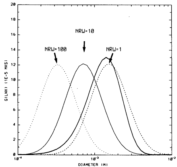
FIG. 2. Mass density functions for a given rainwater content of 0.5 \text{ g m}^{-3} obtained with the log-normal distribution for \sigma = 0.547 and three predicted values of N_{rw} in drops per liter (thin lines) and with the Marshall-Palmer distribution for N_0 = 10^7 \text{ m}^{-4} (thick line).
