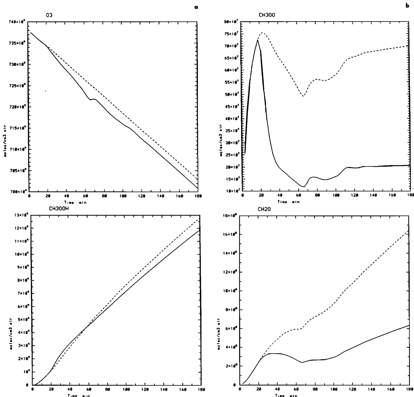
Figure 4. Results of box model runs (a) Ozone and \text{CH}_3\text{O}, \text{H} gas concentrations (at the end of run of 3 hours); (b) \text{CH}_3\text{O} , and \text{CH}_2\text{O} gas concentrations; (c) \text{OH} and \text{HCOOH} gas concentrations; and (d) \text{NO} and \text{NO}_2 gas concentrations; (solid line) 20 microns, (dotted line) 200 microns.
