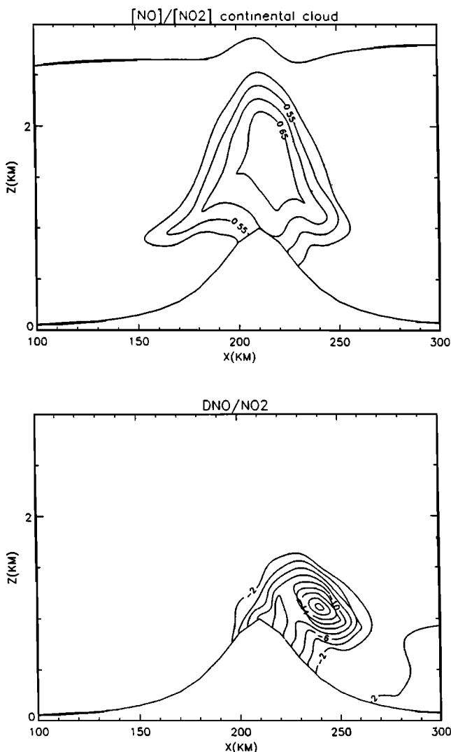
Figure 6. (top) continental cloud; [\text{NO}]/[\text{NO}_2] , (time=3 hours); (bottom) relative difference of the [\text{NO}]/[\text{NO}_2] ratio between the maritime case and the continental case (expressed in percent; continental case taken as reference).
