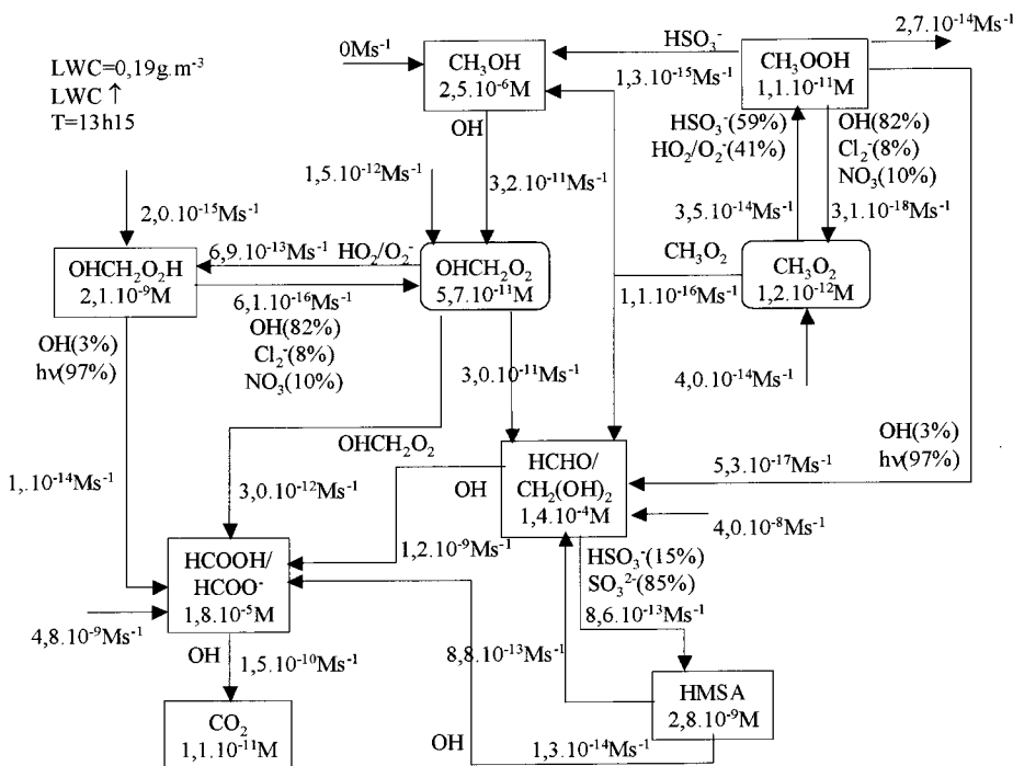
Fig. 5. Concentration/flux diagram for oxidation pathways of COV at 1.15 p.m. (= 13h15) and at LWC = 0.19 g m -3 . Transfer fluxes of 0 M s -1 (methanol) indicate Henry's law equilibrium.
