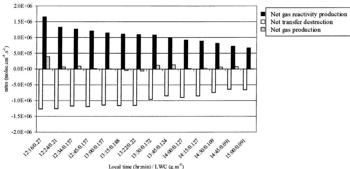
Fig. 8. Source and sink of peroxyoxynitric acid in gas phase for different time and liquid water content during simulation.
