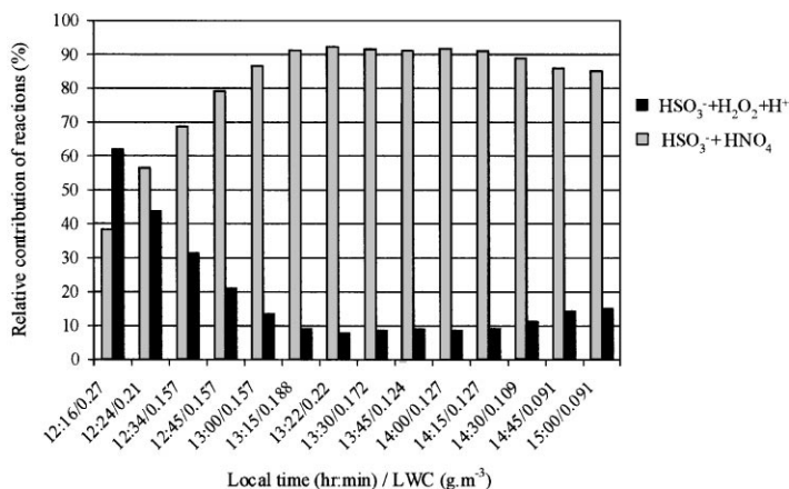
Fig. 7. Production pathways for sulfate at different time and liquid water content during the simulation.
