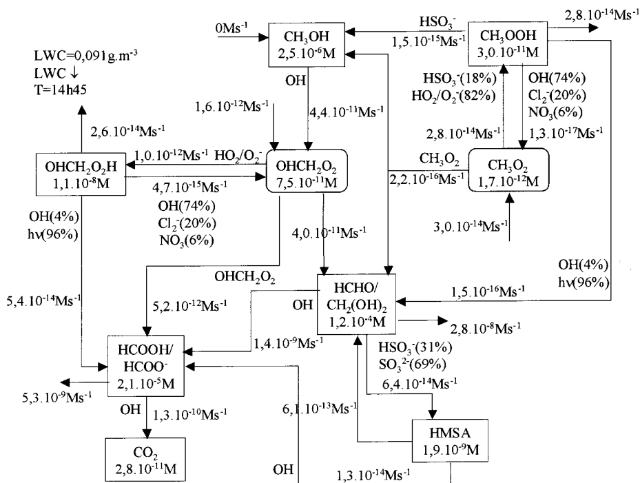
Fig. 6. Same as Fig. 5 but at 2.45 p.m. (=14h45) and at LWC = 0.091 g m -3 .
