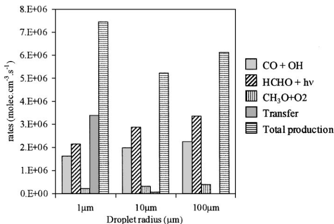
Fig. 4. Rates of gas-phase production of the HO 2 radical at the maximum of the liquid water content (0.22 g m -3 ) at 1.22 p.m. local time for three values of the droplet radius.
