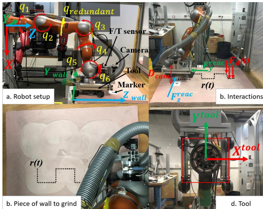
Figure 1: The robotic system equipped with a grinding tool, camera for distance measurement, and a force/torque sensor to perform grinding on a piece of wall
