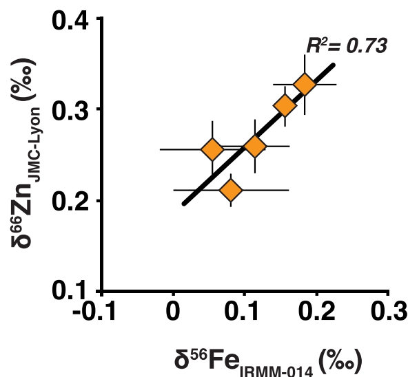
Figure 4. The strong correlation ( R^2 = 0.73 ) between the \delta^{56}\text{Fe} and \delta^{66}\text{Zn} of the basaltic eclogites from the Zermatt-Saas suggest that both the Fe and Zn stable isotopes composition of these samples is controlled by the same process. All errors are 2sd of the mean of n .
