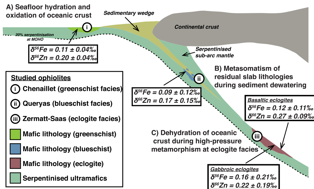
Figure 6. Schematic diagram (modified after Debret et al. [2016a]) showing the approximate location of the meta-ophiolites studied as part of this work: (i) Chenaillet massif; (ii) Queryas complex; and (iii) Zermatt-Saas ophiolite. Each of these meta-ophiolites has been metamorphosed under conditions representative of a subduction gradient (greenschist to blueschist to eclogite) and allows us to examine the effect of slab metamorphism and metasomatism on the mafic oceanic crust. For each of these ophiolites, the average \delta^{56}\text{Fe} and \delta^{66}\text{Zn} values are presented.
