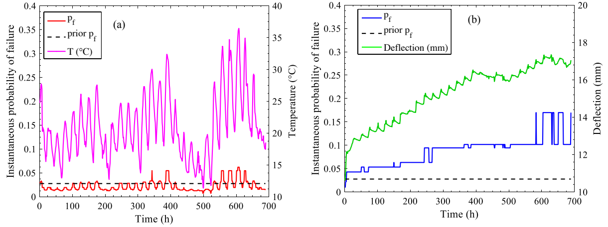
Figure 10: Updating of instantaneous probability of failure with evidences from: (a) Temperature variations only; (b) Deflection variations only.
