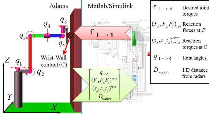
Fig. 6: Adams/Matlab co-simulation
