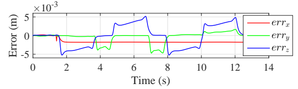
Fig. 8: Position command-response errors
