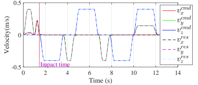
Fig. 9: Velocity command-response
