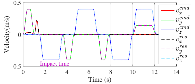
Fig. 9: Velocity command-response
