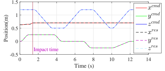
Fig. 7: Position command-response
