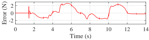
(b) Force command-response error with smooth transition
