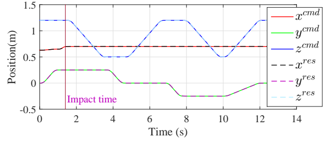
Fig. 7: Position command-response
