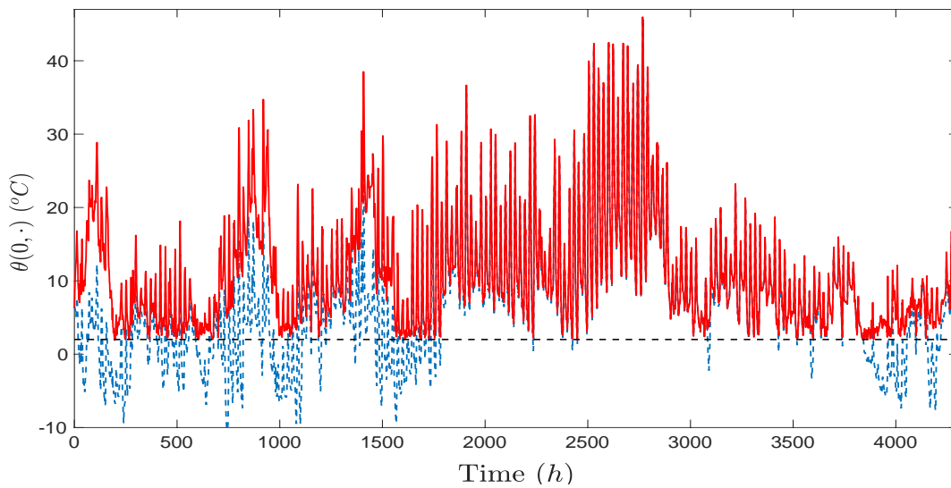
Figure 11: Temperature \theta(0, \cdot) at the road surface on [0, T] in the controlled (red full line) and uncontrolled case (dot blue line).
