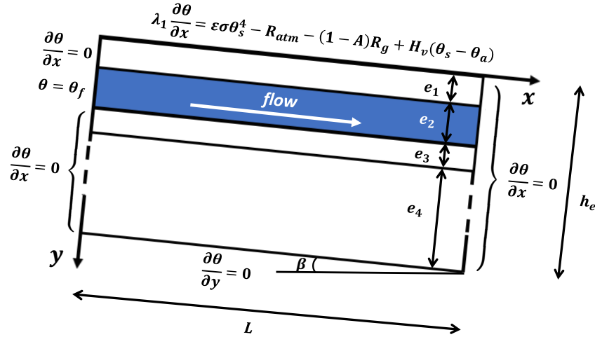
Figure 3: Scheme of pavement structure with its limit conditions ( \theta_f , \theta_a and \theta_s are respectively the injection temperature of the fluid, the air temperature and the road surface temperature).
