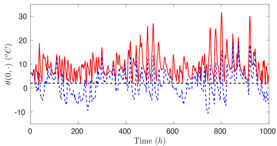
Figure 13: Temperature \theta(0, \cdot) at the road surface on [0, 1000] corresponding to the source q defined by (5.53).
