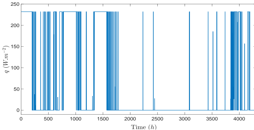
Figure 10: Optimal bang-bang control q on [0, T] corresponding to L = 1/4 . q(t) = \lambda s(t) with \lambda \approx 2.34 \times 10^2 .
