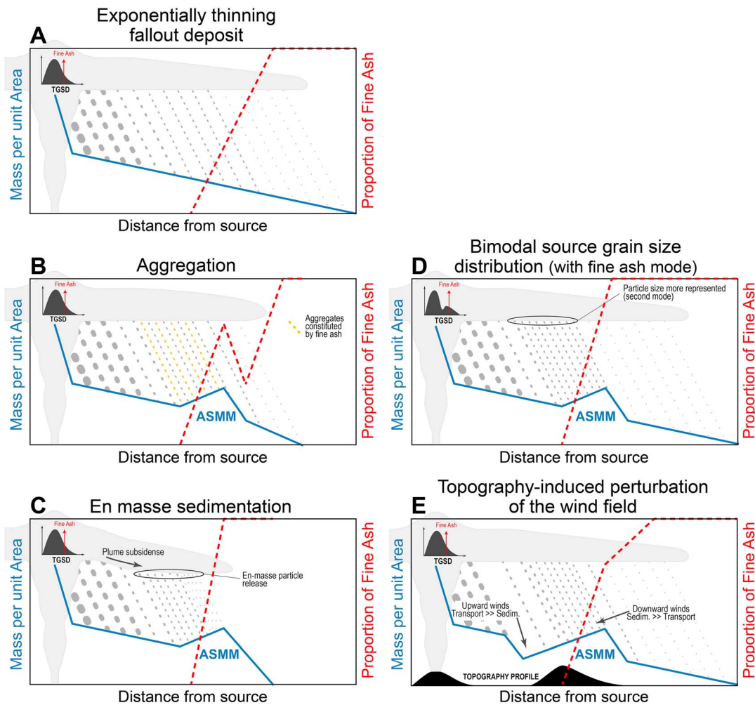
Figure 1. Schematic of the variations of mass and fine ash content (i.e., particles <63 μm in size) in fallout deposits expected for different atmospheric and source conditions, and different sedimentation behaviors. The blue and red dotted lines represent the variations of MpuA (left axis) and proportion of fine ash (right axis), respectively. The cartoons in the background represent schematically the settling of particles from a spreading volcanic plume.
