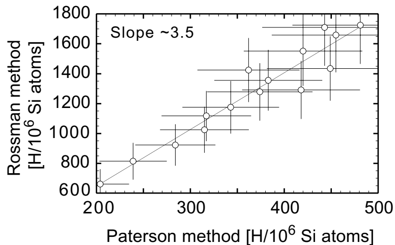
Figure 4. Comparison of H 2 O concentrations in olivine determined by applying two different calculation methods to the same set of FTIR spectra. The method of Paterson [1982] applies variable extinction coefficients to the range of 3650 to 3000 cm -1 . The method of Bell et al. [2002] uses a single extinction coefficient applied to integrated absorption coefficient for the same range. The same geometric correction of 1/2 is applied. Water contents by the method of Bell et al. [2002] are 3.5 times higher on average than those calculated from the method of Paterson [1982]. The higher olivine concentrations were preferred for determining the SIMS calibration for olivine (see text).
