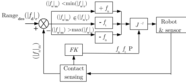
Figure 26: Surface contour following using the contact sensing finger (control diagram). [160]. Range_{des}(|f_d|_r) is a range of the desired force, (|f_n|_m) is the measured normal force, (|f_n|_r) is the friction cone, (f_n) and (f_t) are the normal and tangential forces, P is the contact point location, and (J^{-1}) is the robot's inverse kinematics.
