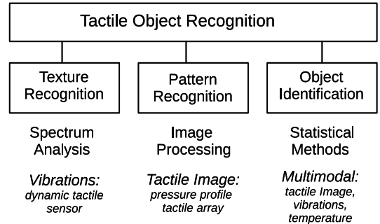
Figure 19: Tactile object recognition. Tactile data can be used for classification of textures based on spectrum of frequencies that appear during the sliding over a surface [43]. Object that is in contact with the tactile sensing array can be recognized from the contact patterns using image processing techniques [40]. When multimodal tactile information is available, objects can be identified through statistical and probabilistic analysis of multimodal data [19].
