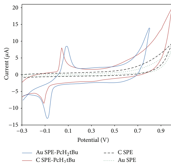
FIGURE 2: CV studies of the modified electrodes revealing the redox peaks of the \text{PcH}_2\text{tBu} in KCl 0.1M. For comparison the cyclic voltammogram of the bare electrodes on the KCl solution are shown.
