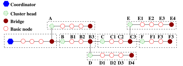
Figure 2: A Long Thin WSN as proposed in [9]
