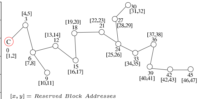
Figure 12: Simple topology discovered by TopoProto
