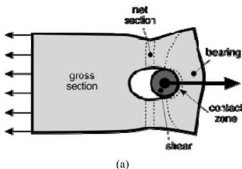
Fig. 3 Zones of deformation (a); joint with two bolts in shear showing large hole elongation after test (b)
