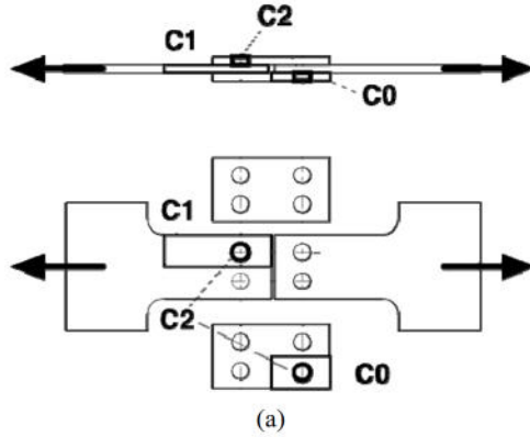
Fig. 4 Cover-plate joint components for modeling (a); deformed components C0 and C1 (b)
