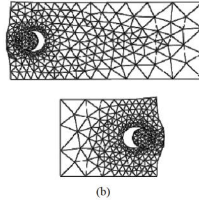
Fig. 4 Cover-plate joint components for modeling (a); deformed components C0 and C1 (b)
