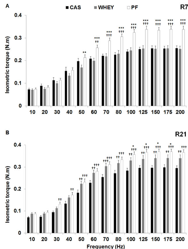
Figure 3. Recovery kinetics of the torque-frequency relationship: torque-frequency relationship after 7 (R7; panel A) and 21 days (R21; panel B) of recovery in the experimental groups fed with casein (CAS; black bars), whey (WHEY; grey bars), and in the pair-fed control group (PF; white bars). Significantly different from WHEY: **: P < 0.01 ; ***: P < 0.001 . Significantly different from CAS: ††: P < 0.01 ; †††: P < 0.001 . doi:10.1371/journal.pone.0075408.g003
