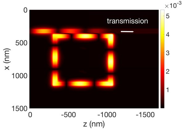
FIG. 6. Modulus of H_y(x, z) at frequency 296.6 THz, for g = 25 nm. Numerical parameters: L_x = L_z = 725 nm, g = 25 nm, d = 50 nm.
