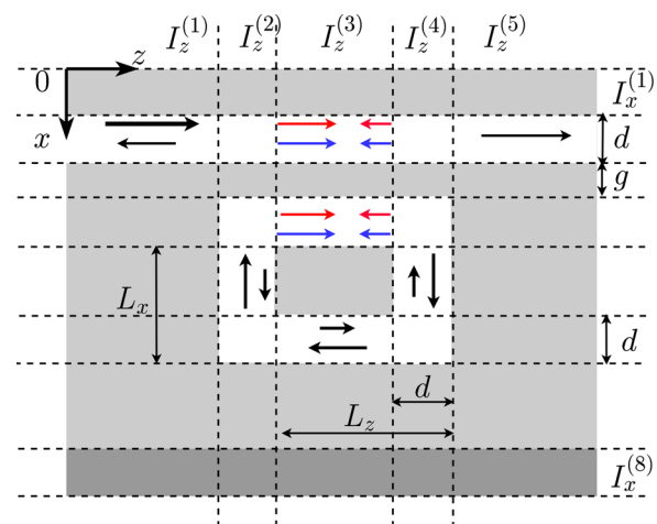
FIG. 1. Schematic of a plasmonic rectangular MIM resonator. Illustration of the staircase concatenation of the MIM resonator according to the ( Oz ) and ( Ox ) directions. The structure is divided into five layers I_z^{(k)} , k = 1 : 5 in the ( Oz ) direction and height intervals I_x^{(k)} , k = 1 : 8 in the ( Ox ) direction. The layers I_z^{(1)} (resp. I_z^{(5)} ) correspond to the input (resp. output) waveguide bus.
