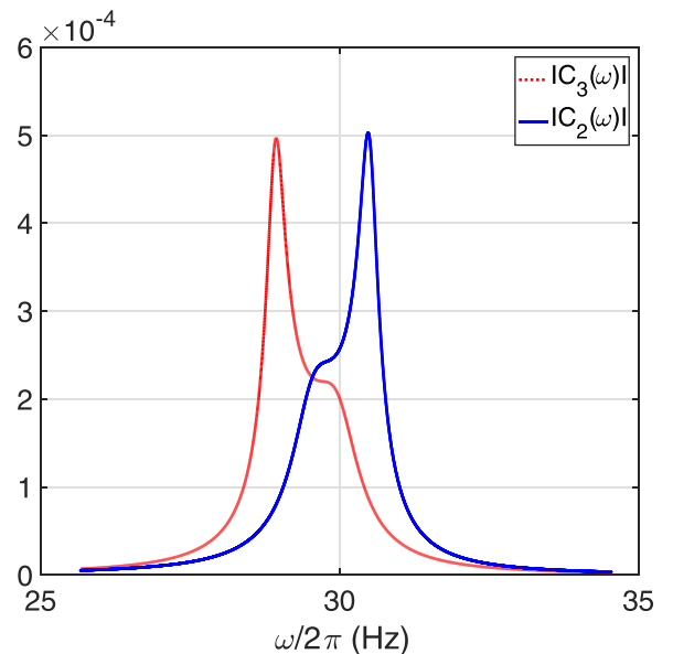
FIG. 9. Fano resonance illustration with two coupled oscillators. Numerical parameters: \omega_1/2\pi = 2.93 , \omega_2/2\pi = 2.99 , \omega_3/2\pi = 3.04 , \omega_4/2\pi = 3.09 , \gamma_1 = \gamma_4 = 0.2 , \gamma_2 = \gamma_3 = 0.5 , \nu_{13} = \nu_{31} = \nu_{14} = \nu_{41} = 0.05 , a_1 = 1 = a_4 = 1 .
