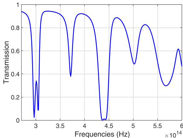
FIG. 2. Transmission spectrum of the MIM resonator. Numerical parameters: L_x = L_z = 725 nm, g = 25 nm, d = 50 nm.
