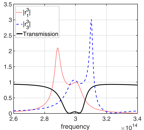
FIG. 13. Transmission spectra ( \omega/2\pi \in [260, 340] THz) of the MIM resonator for g = 20 . Other Numerical parameters: L_x = L_z = 725 nm, d = 50 nm.
