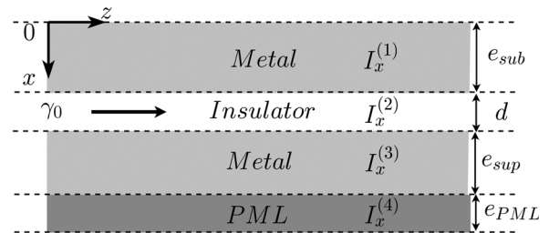
FIG. 3. Illustration of the numerical configuration for the modal analysis of MIM waveguide. The structure is subdivided into four homogeneous domains (intervals) ( I_x^{(1)}, I_x^{(2)}, I_x^{(3)}, I_x^{(4)} ) along the ( Ox ) axis with the thickness ( e_{sub}, d, e_{sup}, e_{pml} ).
