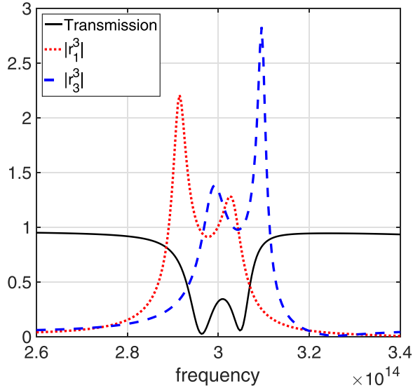
FIG. 14. Transmission spectra ( \omega/2\pi \in [260, 340] THz) of the MIM resonator for g = 25 . Other Numerical parameters: L_x = L_z = 725 nm, d = 50 nm.
