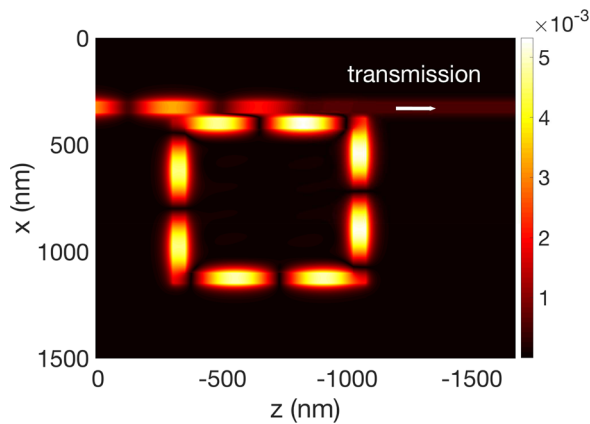
FIG. 8. Modulus of H_y(x, z) at frequency 304.4 THz, for g = 25 nm. Numerical parameters: L_x = L_z = 725 nm, g = 25 nm, d = 50 nm.
