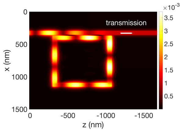
FIG. 7. Modulus of H_y(x, z) at frequency 301.2 THz, for g = 25 nm. Numerical parameters: L_x = L_z = 725 nm, g = 25 nm, d = 50 nm.
