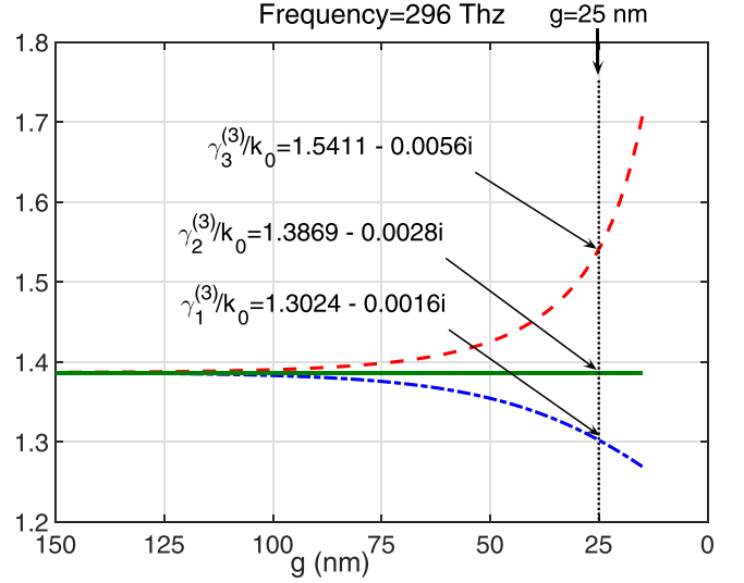
FIG. 4. Illustration of the lift of degeneracy of eigenmodes of the superstructure for g \in [15, 145] nm. Numerical parameters: frequency = 296 THz, L_x = 725 nm, d = 50 nm.
