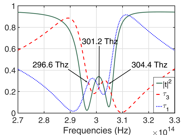
FIG. 5. Normalized forward power spectra \tau_1 (resp. \tau_3 ) associated with the eigenmode \gamma_1^{(3)} (resp. \gamma_3^{(3)} ) for g = 25 nm. Numerical parameters: L_x = L_z = 725 nm, d = 50 nm.
