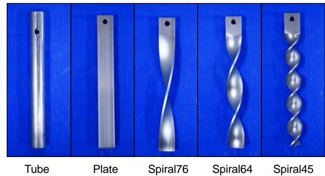
Fig. 1. Model piles.
