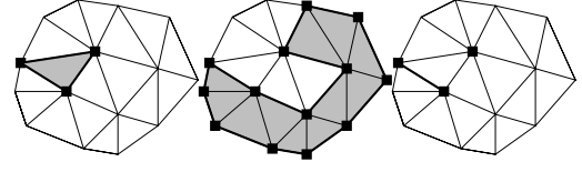
Fig. 2 Lemma 1 in the 2D case. Left: c(\Delta) and c(\partial\Delta) . Middle: c(O) and c(\partial O) . Right: c(\Delta) \cap c(O) . Both \Delta and O are in gray, T is the set of all triangles, \Delta \in T \setminus O , the edges of c(\partial\Delta) and c(\partial O) are thickened, the vertices of c(\Delta) and c(O) are black squares. We see that c(\Delta) \cap c(O) has 1 edge and 3 vertices, c(\Delta) \cap c(O) = c(\partial\Delta) \cap c(\partial O) , \partial O \cap \partial\Delta has 1 edge.
