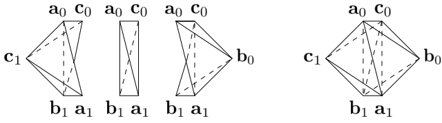
Fig. 12 The pipe p(a_0b_0c_0, a_1b_1c_1) (right) and its decomposition (left). See the internal tetrahedron a_0a_1b_1c_0 .
