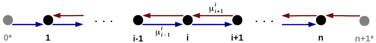
Figure 3: Formation graph with virtual leaders (*) and control coefficients
