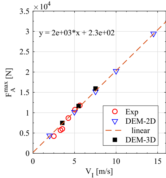
Figure 2. Maximal measured force F_A^{max} obtained by experimental test ( \circ ), simulation tests in 2D ( \nabla ) [2] and simulation tests in 3D ( \square ).
