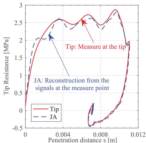
Figure 4. Validation of applied theories on Panda 3®: Tip : tip resistance measured directly at the tip; JA : tip resistance calculated from the force F_A and acceleration Acc_A at the measurement point A
