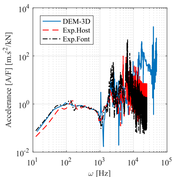
Figure 5. Comparaison of accelerance curve A/F(\omega) obtained by the numerical model (DEM-3D) and by experimental tests of Panda 3® for Hostun (Exp.Host) and Fontainebleau sands (Exp.Font) for tip resistance values around 2 MPa
