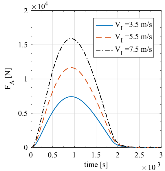
Figure 1. Force F_A at the measuring point A versus time for different impact velocities ( V_I ) with rod length L_t = 8m .
