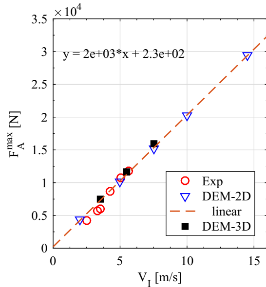
Figure 2. Maximal measured force F_A^{max} obtained by experimental test ( \circ ), simulation tests in 2D ( \nabla ) [2] and simulation tests in 3D ( \square ).
